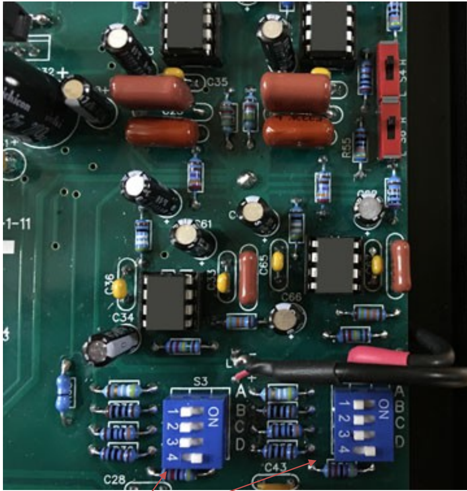
DIP switches for resistive loading
