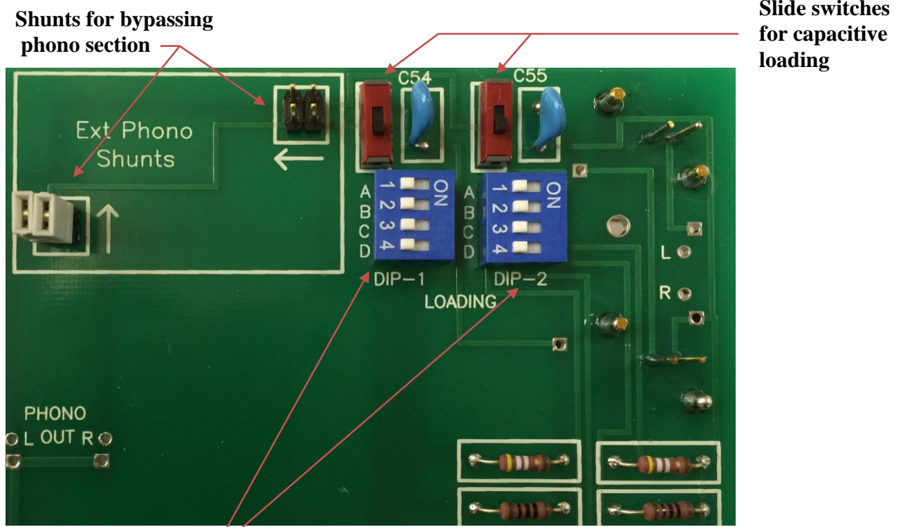
DIP switches for resistive loading
